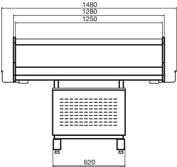
Stella H100 125
