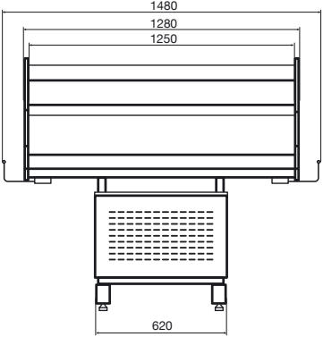
Stella H120 125
