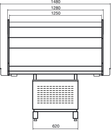
Stella H130 125
